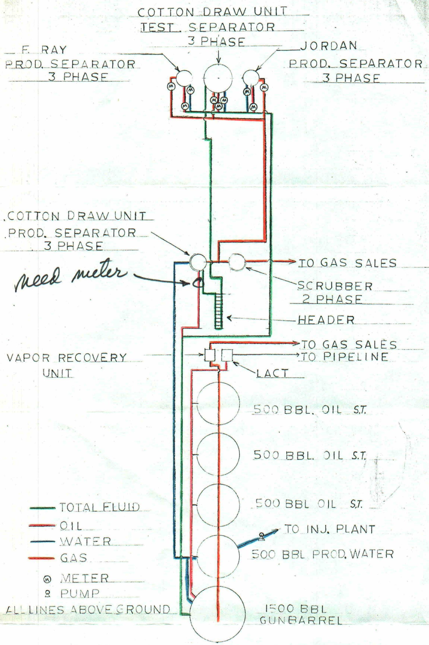
TEXACO INC. PADUCA DELAWARE FIELD SCHEMATIC DIAGRAM OF THE PROPOSED COMMINGLING FACILITY
