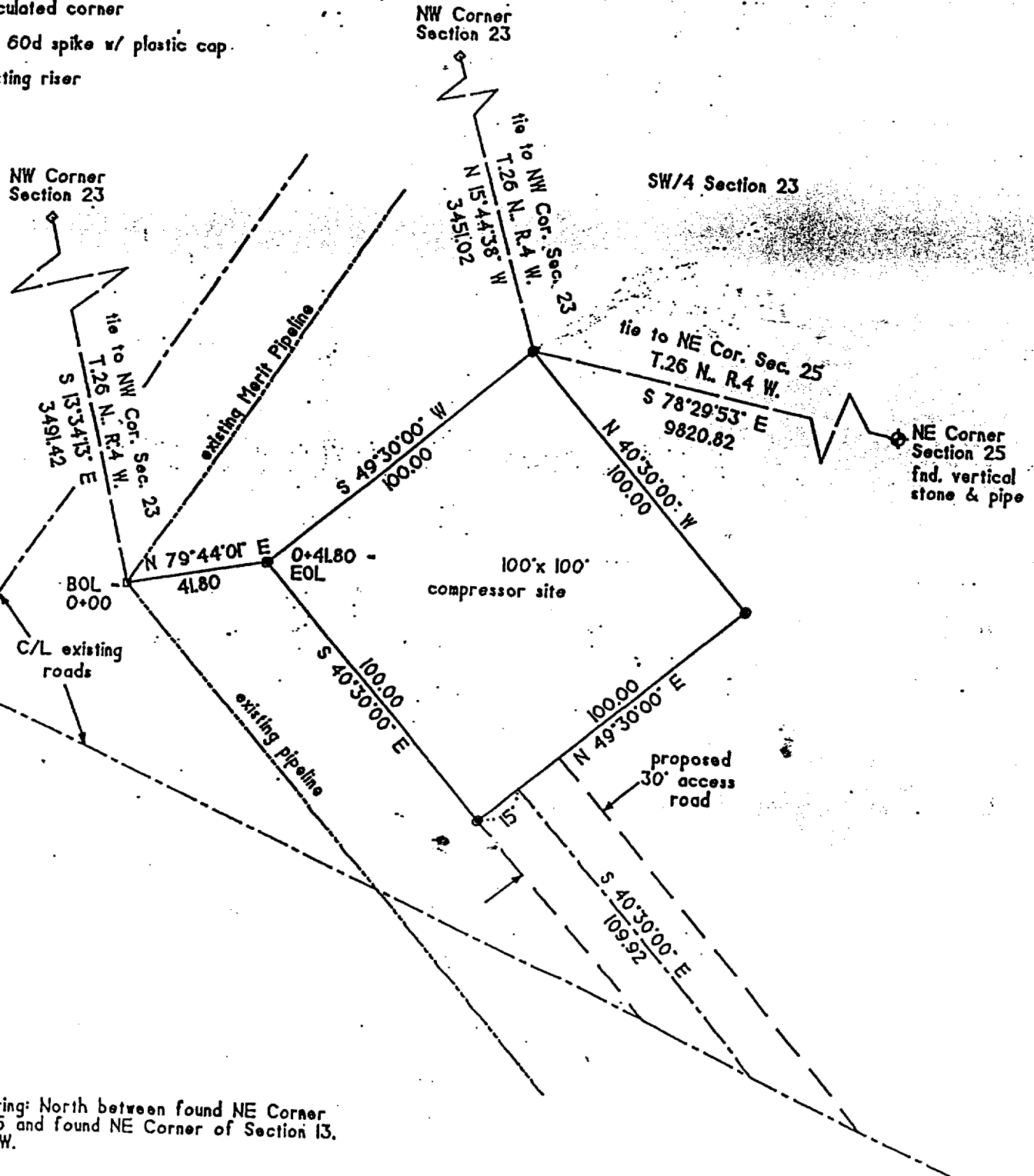
Figure 3. A-Ridge Compressor plat, prepared by Huddleston Land Surveying.
