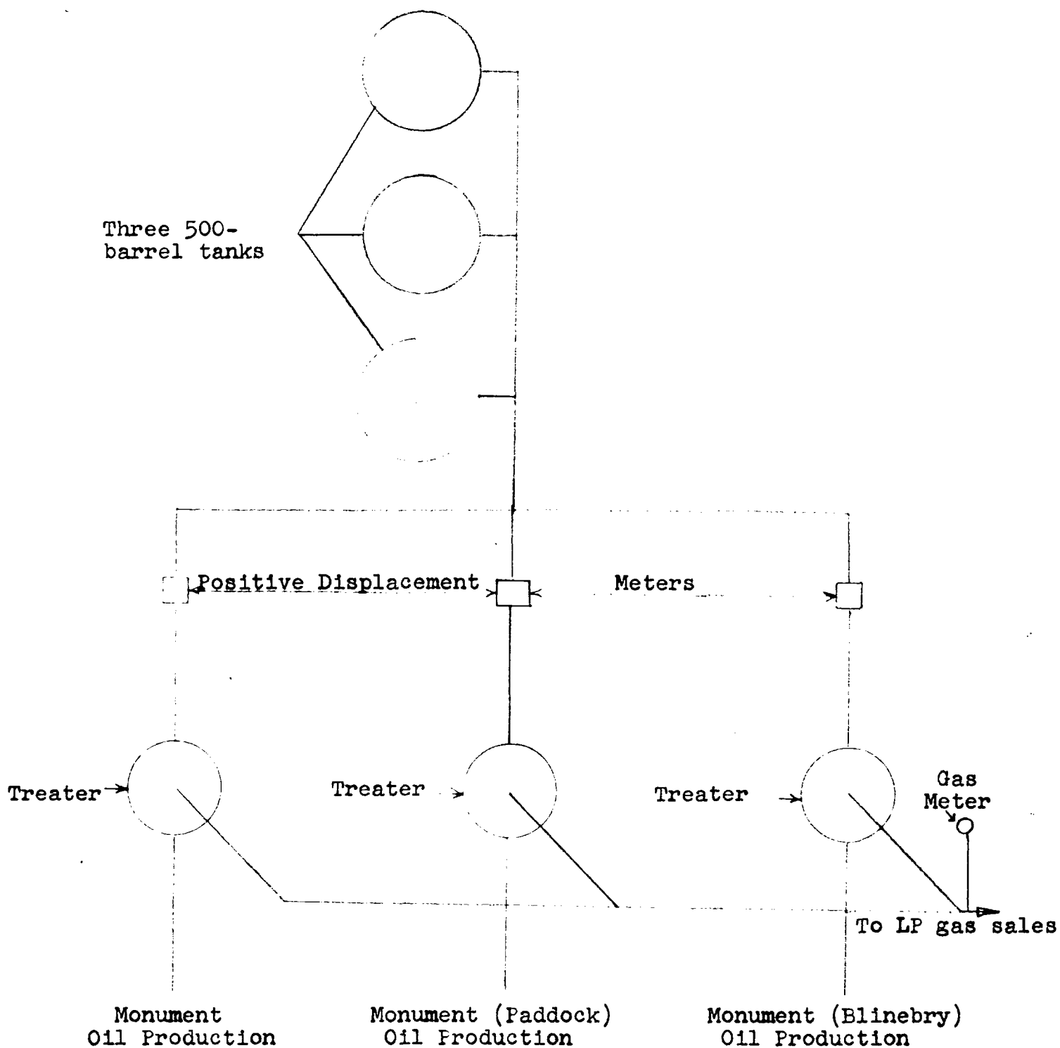
Schematic Diagram of Commingling Installation TEXACO Inc. J. R. Phillips Lease Monument, Monument (Paddock) and Monument (Blinebry) Pools NW/4 Section 6, T-20-S, R-37-E Lea County, New Mexico
