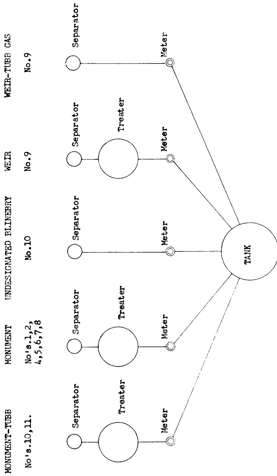
CONTINENTAL OIL COMPANY Schematic Diagram of PROPOSED INSTALLATION BRITT B-15 LEASE
