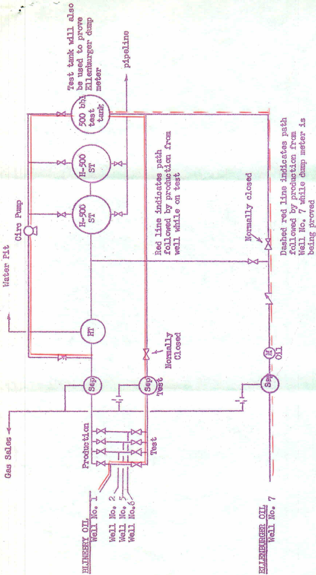
SCHEMATIC DIAGRAM PROPOSED COMINGLING INSTALLATION SCARBOROUGH ESTATE LEASE
