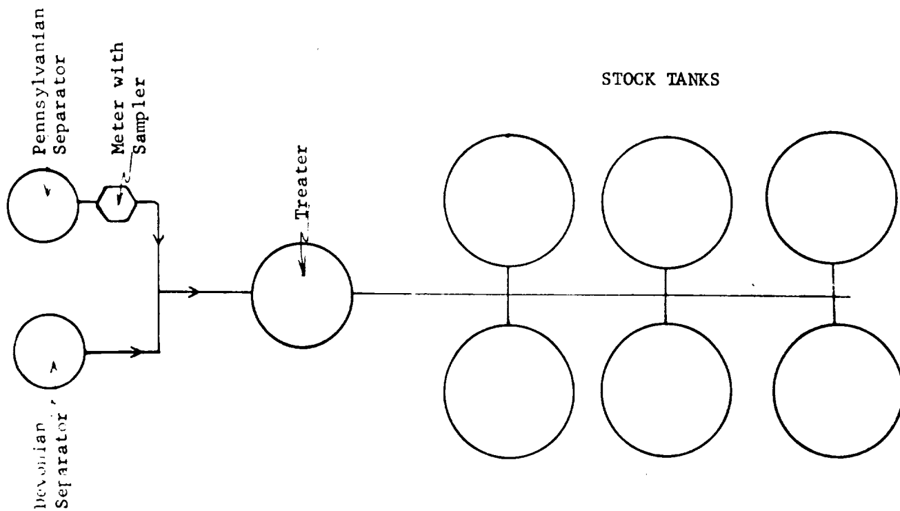
Diagram of Surface Equipment
