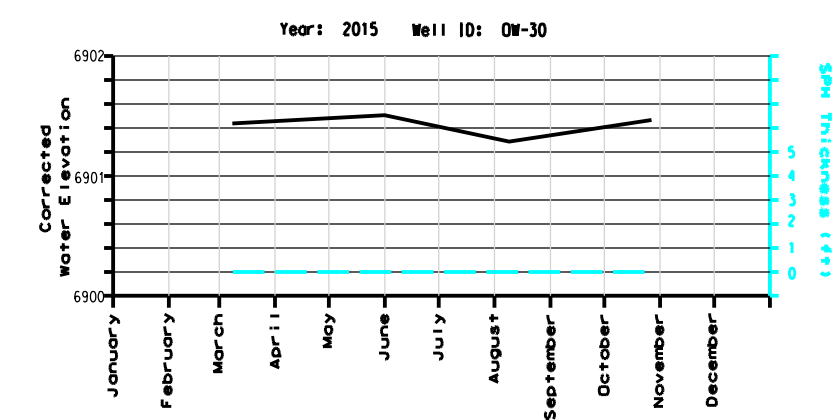
Figure 11 GROUNDWATER ELEVATION VS TIME - 2015 WESTERN REFINING - GALLUP REFINERY
