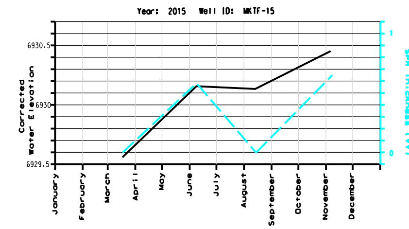
Figure 11.1 GROUNDWATER ELEVATION VS TIME - 2015 WESTERN REFINING - GALLUP REFINERY
