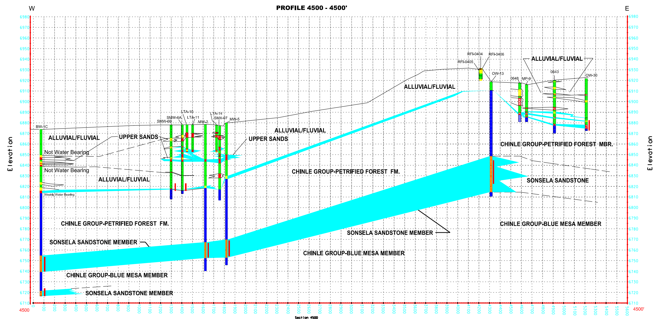
Figure 14 TYPICAL WEST - EAST GEOLOGIC PROFILE WESTERN REFINING - GALLUP REFINERY
