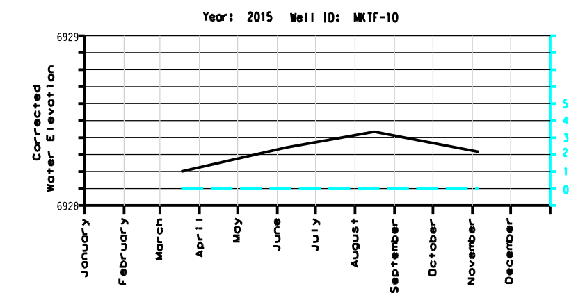
Figure 11.1 GROUNDWATER ELEVATION VS TIME - 2015 WESTERN REFINING - GALLUP REFINERY
