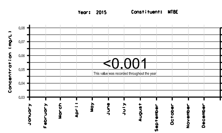
Figure 17.9 WELL GROUP E CONSTITUENTS - 2015 WESTERN REFINING - GALLUP REFINERY
