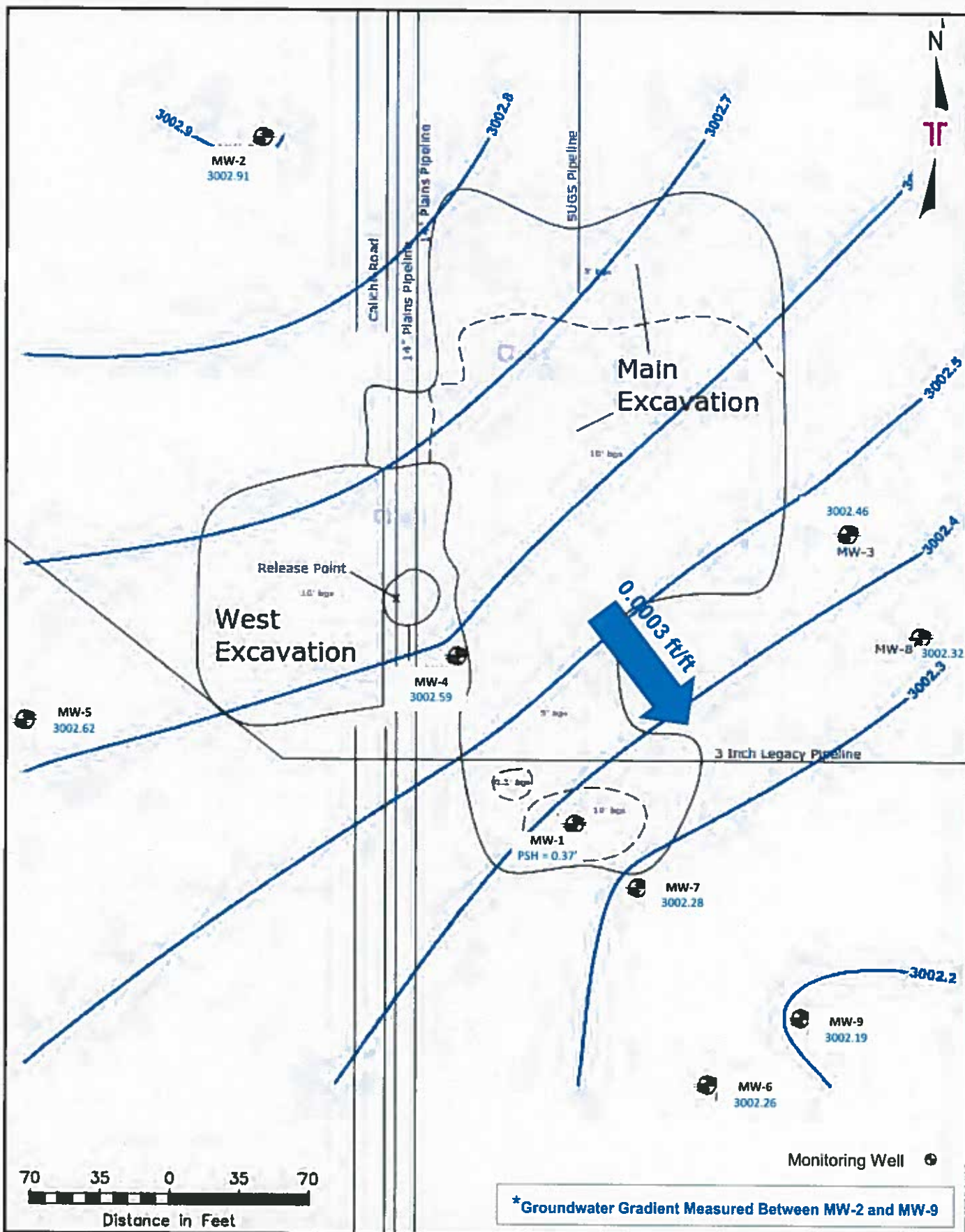
Figure 2a – Groundwater Gradient Map -1Q2017
