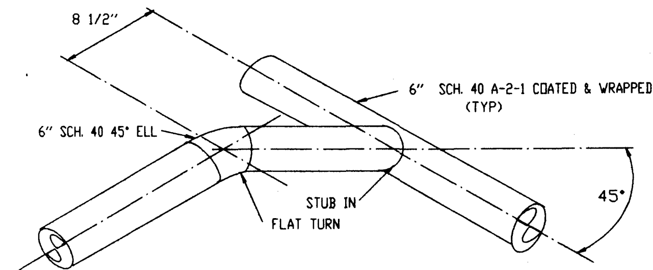
DETAIL #1 THIS DWG. (TYP. FOR S) NOTE: ALL 6" PIPE TURNS SIMILAR.
