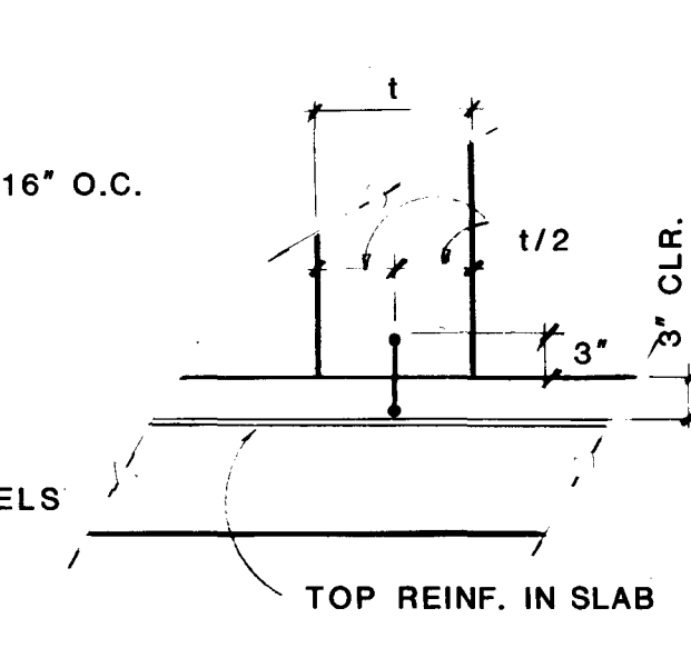
DETAIL A SCALE: 3/4" 1'-0"
