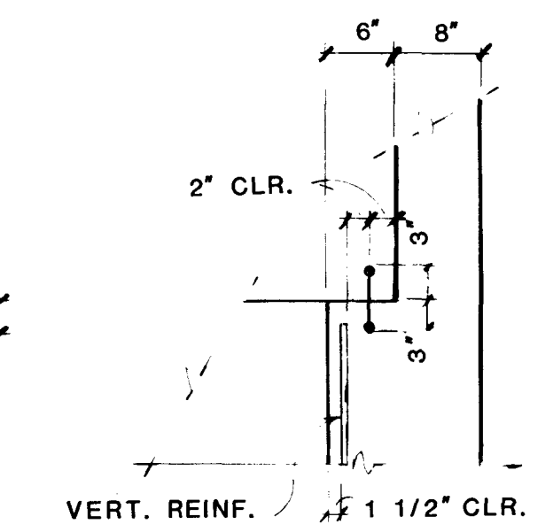
DETAIL B SCALE: 3/4" 1'-0"
