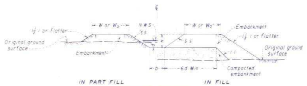
UNLINED SECTION ( d < 2.0' )
