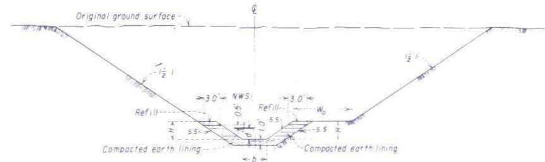
EARTH LINED SECTION IN THOROUGH CUT ( d < 2.0' )
