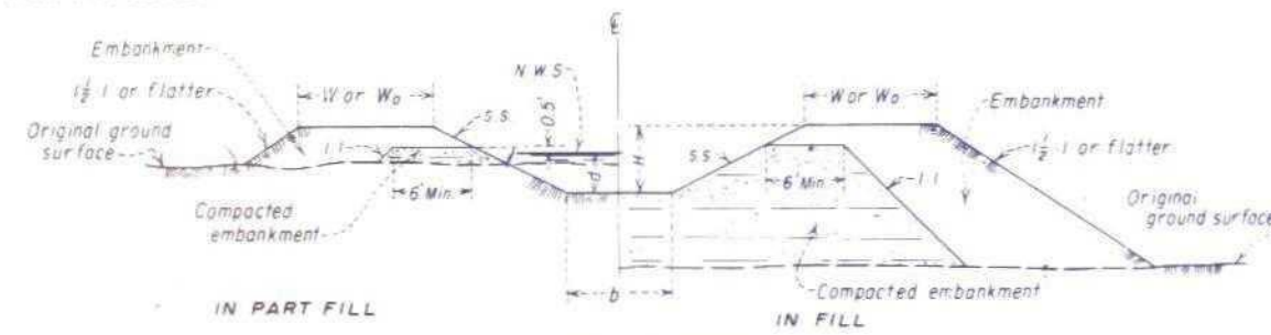
UNLINED SECTION ( d > 2.0' )
