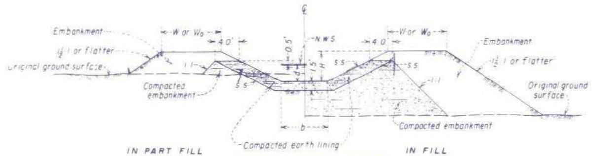
EARTH LINED SECTION ( d > 2.0' )
