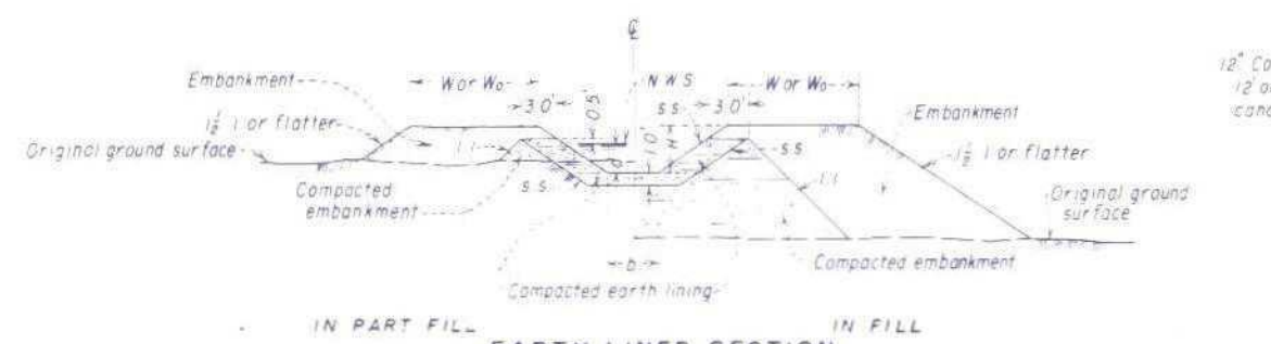
EARTH LINED SECTION ( d < 2.0' )
