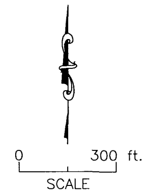
FIGURE 3 POTENTIOMETRIC SURFACE JULY 25, 2000
