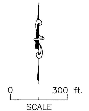
FIGURE 3 POTENTIOMETRIC SURFACE JULY 25, 2000
