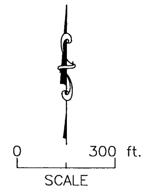
FIGURE 4 TOTAL HALOCARBONS CONCENTRATION MAP JULY 25, 2000
