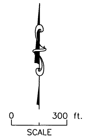
FIGURE 3 POTENTIOMETRIC SURFACE MAP (10/20/99)
