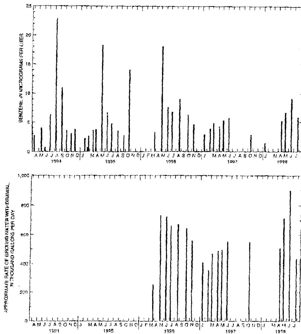
Figure 2.--Concentrations of benzene in water from well 25 as a function of time and approximate rates of ground water withdrawal from well 25 as a function of time (data from City of Hobbs, New Mexico).
