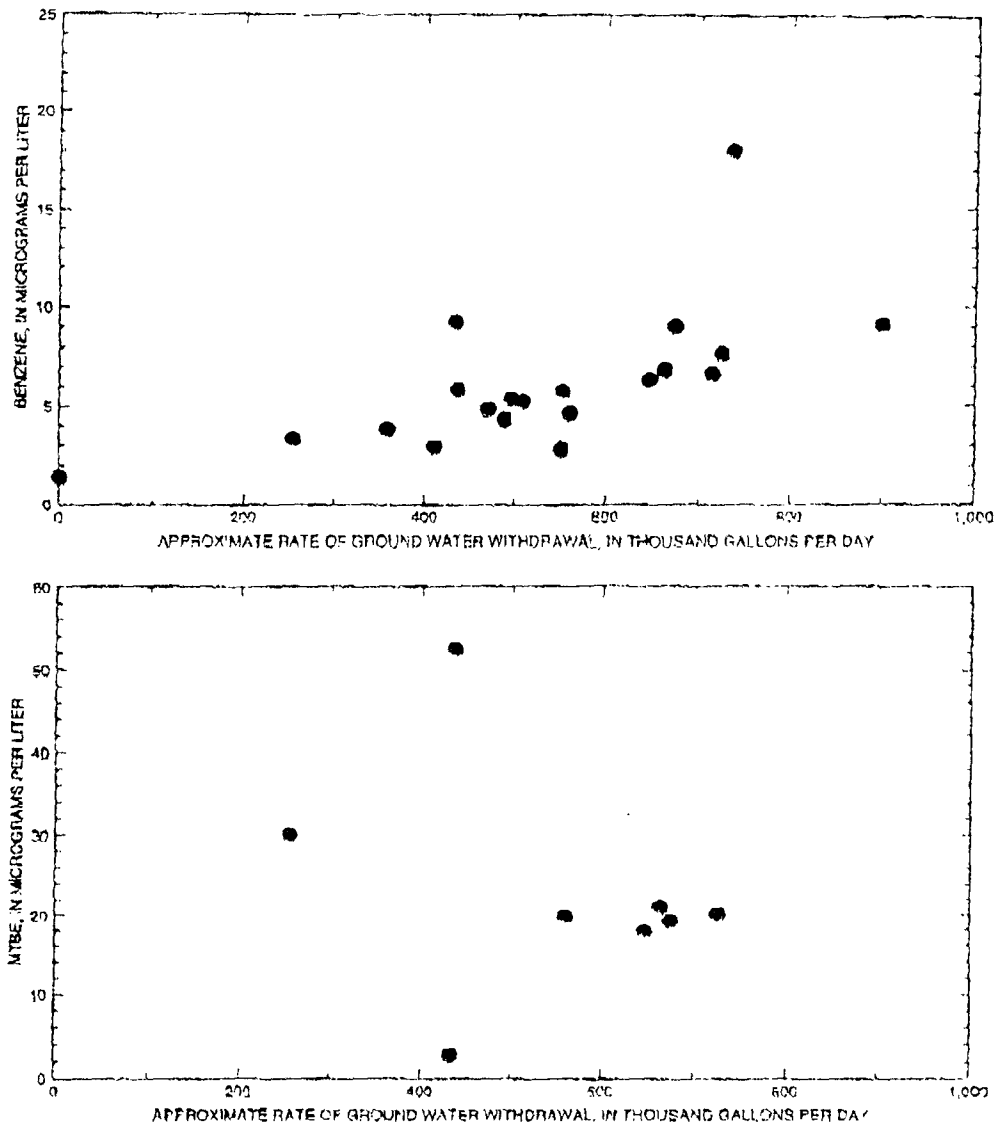
Figure 3.--Concentrations of benzene and MTBE in water from well 25 as a function of approximate rates of ground water withdrawal from well 25 for the period of March, 1996 to August, 1998 (data from City of Hobbs, New Mexico).
