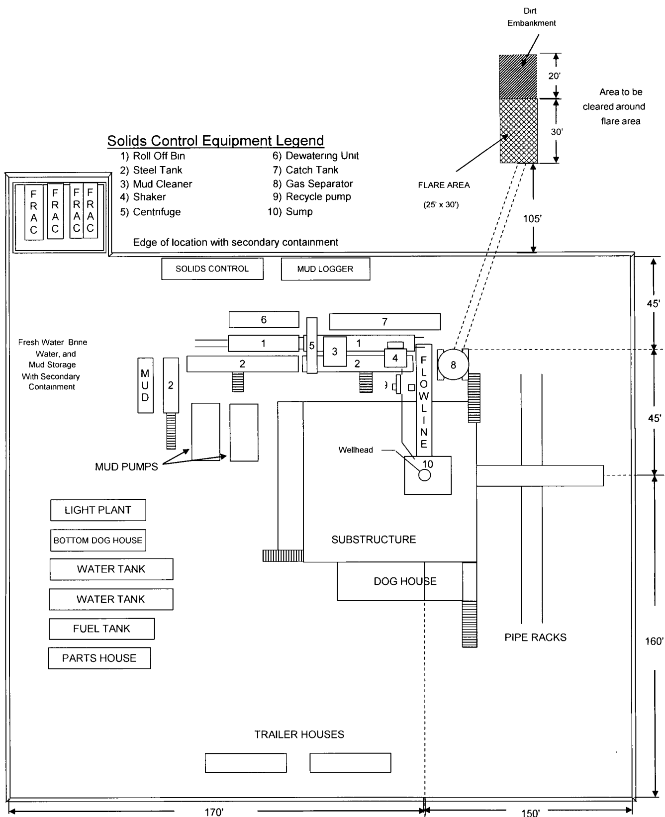
POKER LAKE UNIT 328H TYPICAL RIG LAYOUT SCHEMATIC INCLUSIVE OF CLOSED-LOOP DESIGN PLAN
