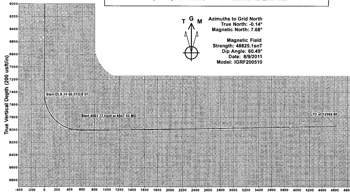
Vertical Section at 0.07° (200 usft/in)
