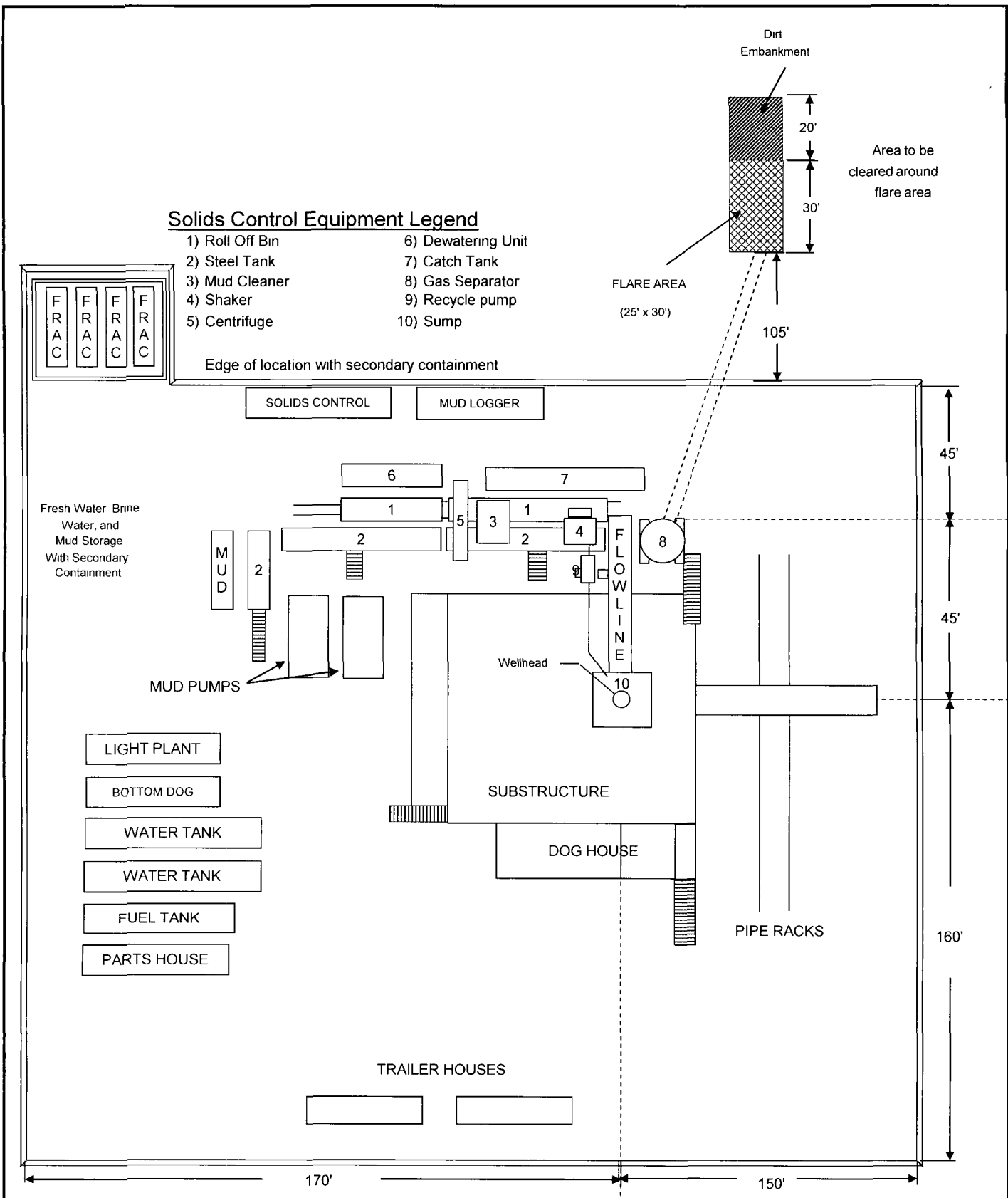
POKER LAKE UNIT 335H TYPICAL RIG LAYOUT SCHEMATIC INCLUSIVE OF CLOSED-LOOP DESIGN PLAN
