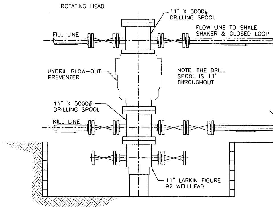
WELLHEAD ELEVATION
