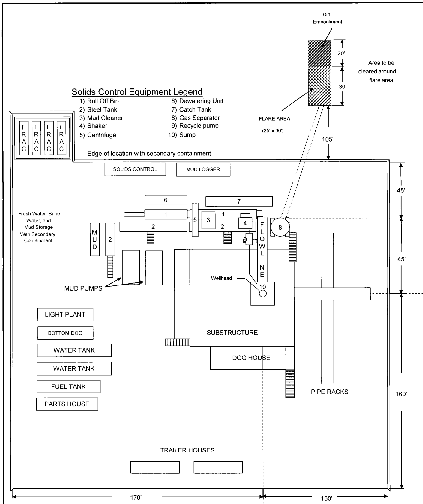
POKER LAKE UNIT 325H TYPICAL RIG LAYOUT SCHEMATIC INCLUSIVE OF CLOSED-LOOP DESIGN PLAN
