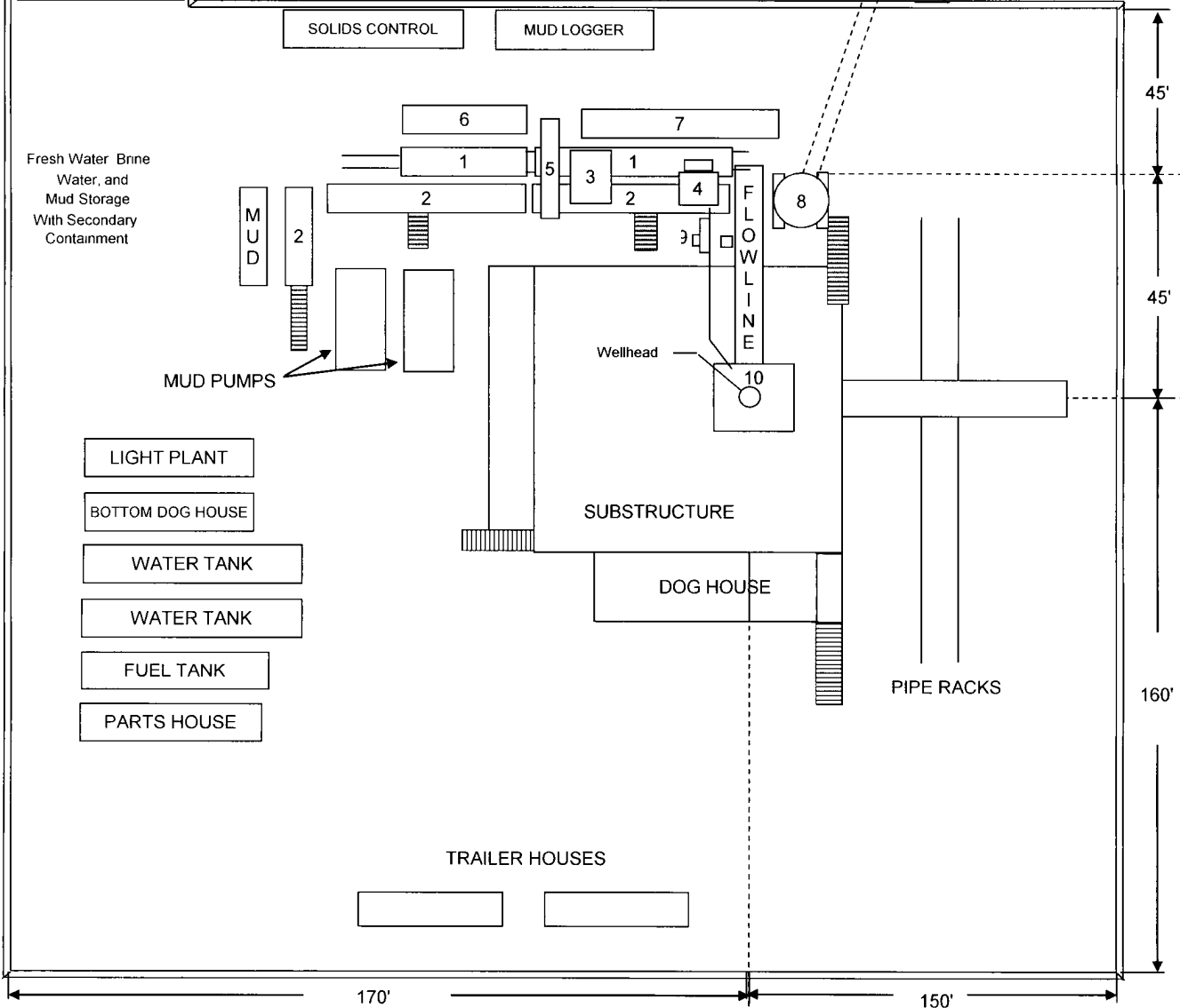
POKER LAKE UNIT 346H TYPICAL RIG LAYOUT SCHEMATIC INCLUSIVE OF CLOSED-LOOP DESIGN PLAN
