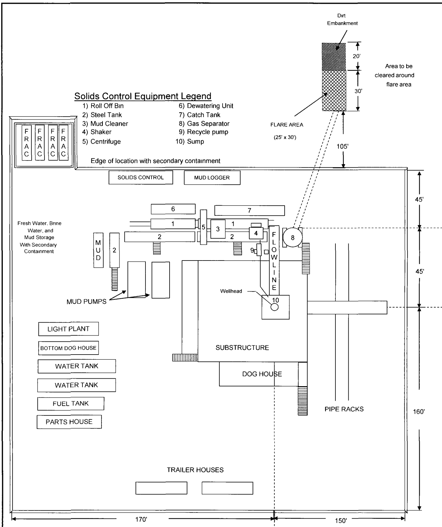
POKER LAKE UNIT 344H TYPICAL RIG LAYOUT SCHEMATIC INCLUSIVE OF CLOSED-LOOP DESIGN PLAN
