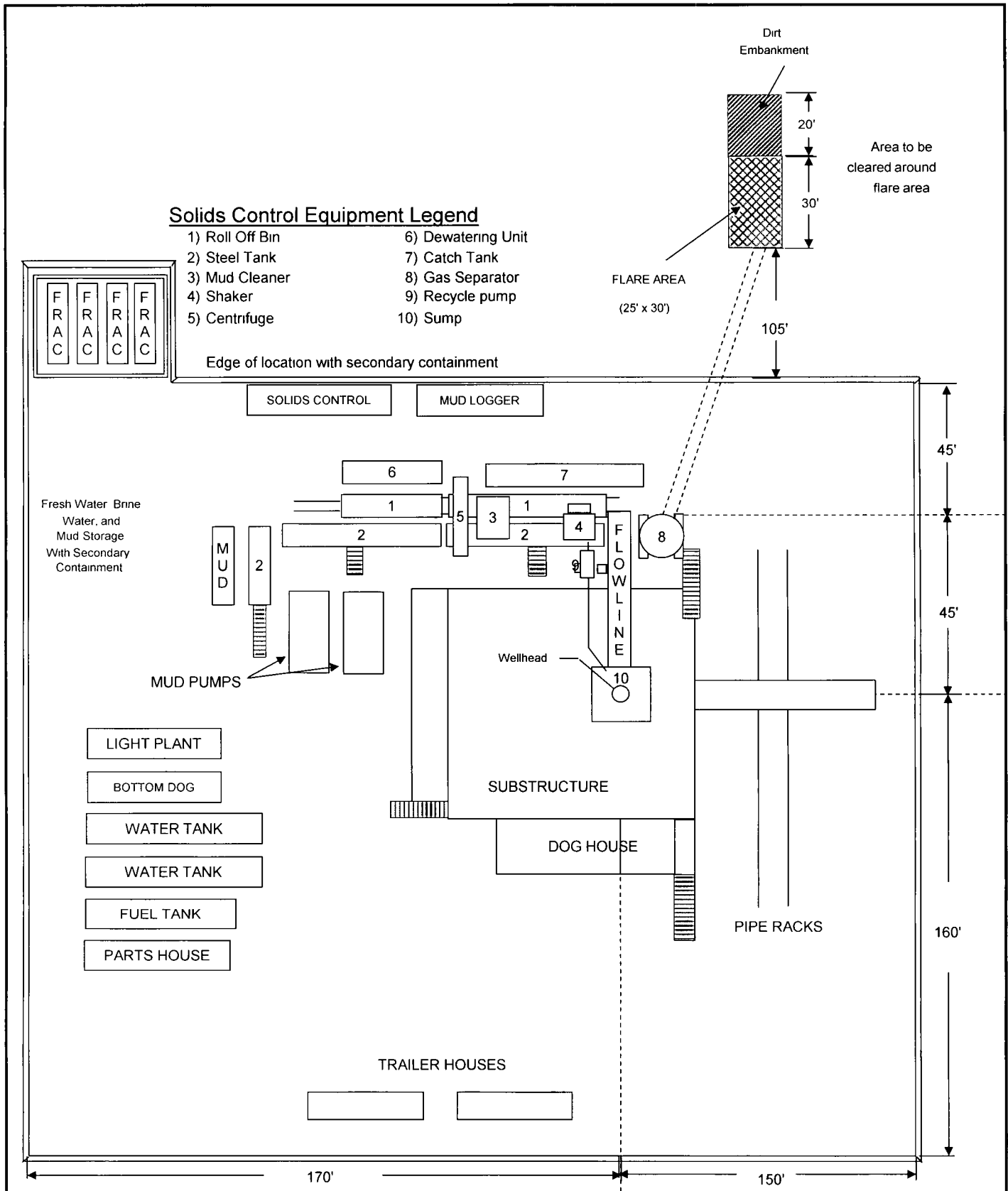
POKER LAKE UNIT 320H TYPICAL RIG LAYOUT SCHEMATIC INCLUSIVE OF CLOSED-LOOP DESIGN PLAN
