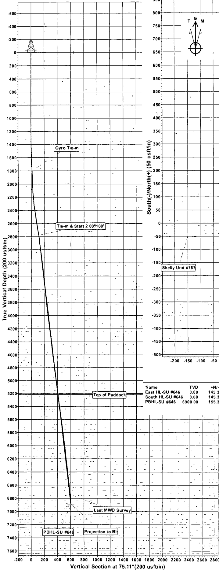
PROJECT DETAILS: Eddy County, NM (NAN27 NME) Plan: Plan #2 - 7-7/8" Hole (Skelly Unit #646/OH)
