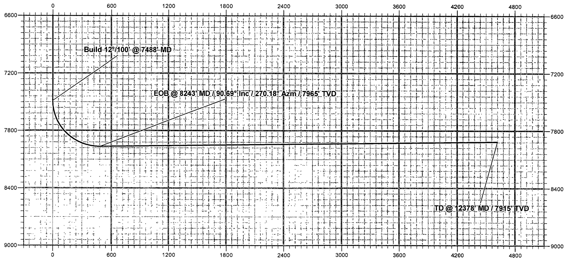
Vertical Section at 270.18° (600 usft/in)
