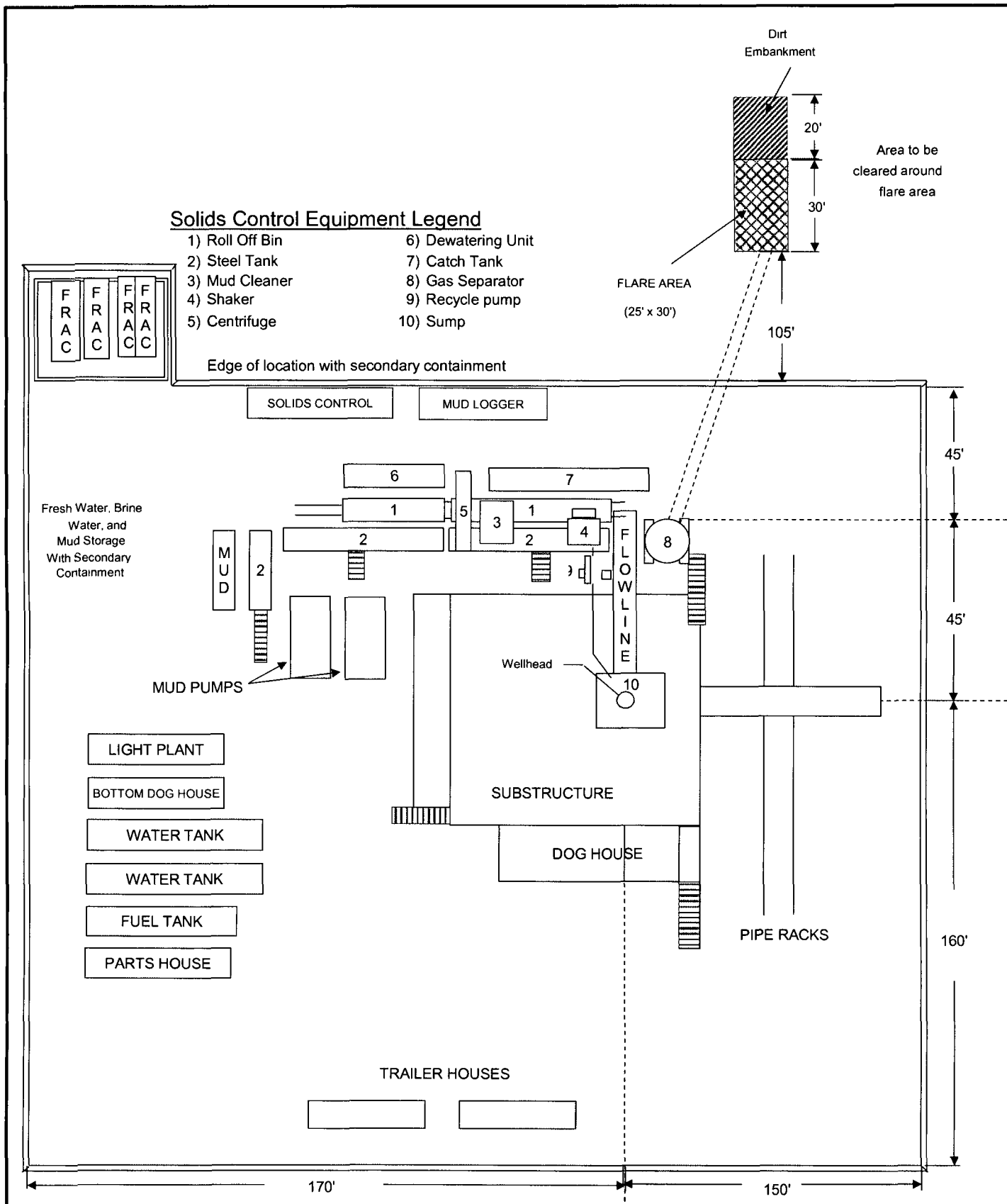
BEU HACKBERRY 34 FEDERAL 1 SWD TYPICAL RIG LAYOUT SCHEMATIC INCLUSIVE OF CLOSED-LOOP DESIGN PLAN
