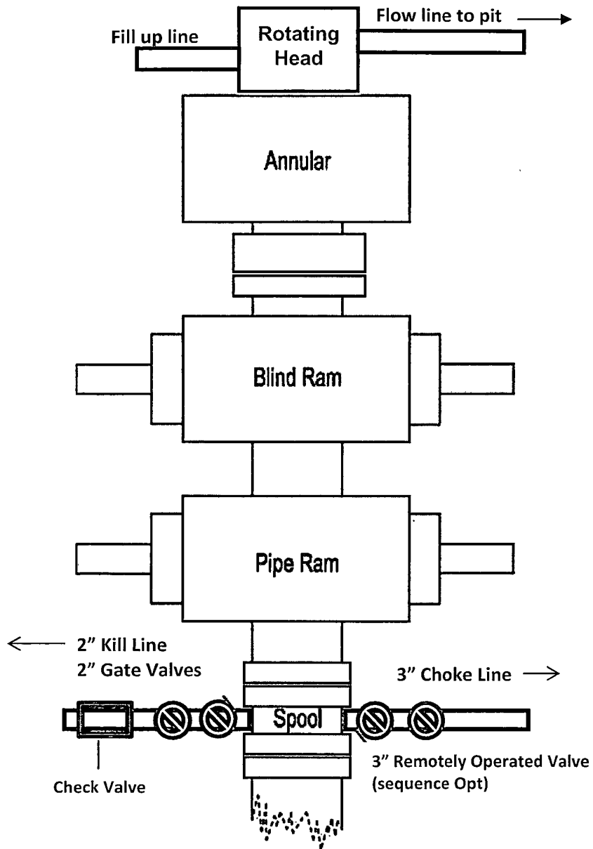
3M psi BOPE & Choke Manifold Exhibit 3 All valve & lines on choke manifold are 2" unless noted. Exact manifold configuration may vary
