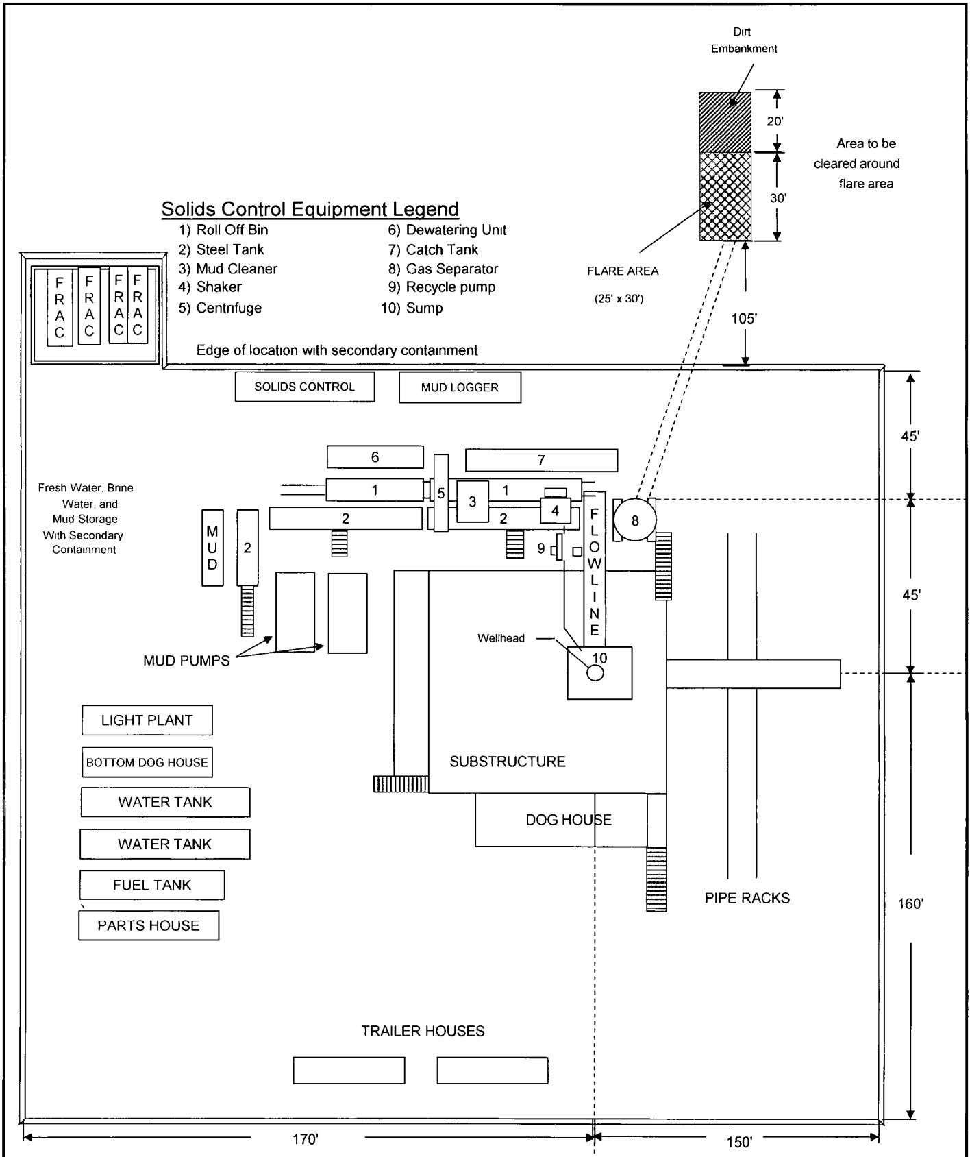
POKER LAKE UNIT 415H TYPICAL RIG LAYOUT SCHEMATIC INCLUSIVE OF CLOSED-LOOP DESIGN PLAN
