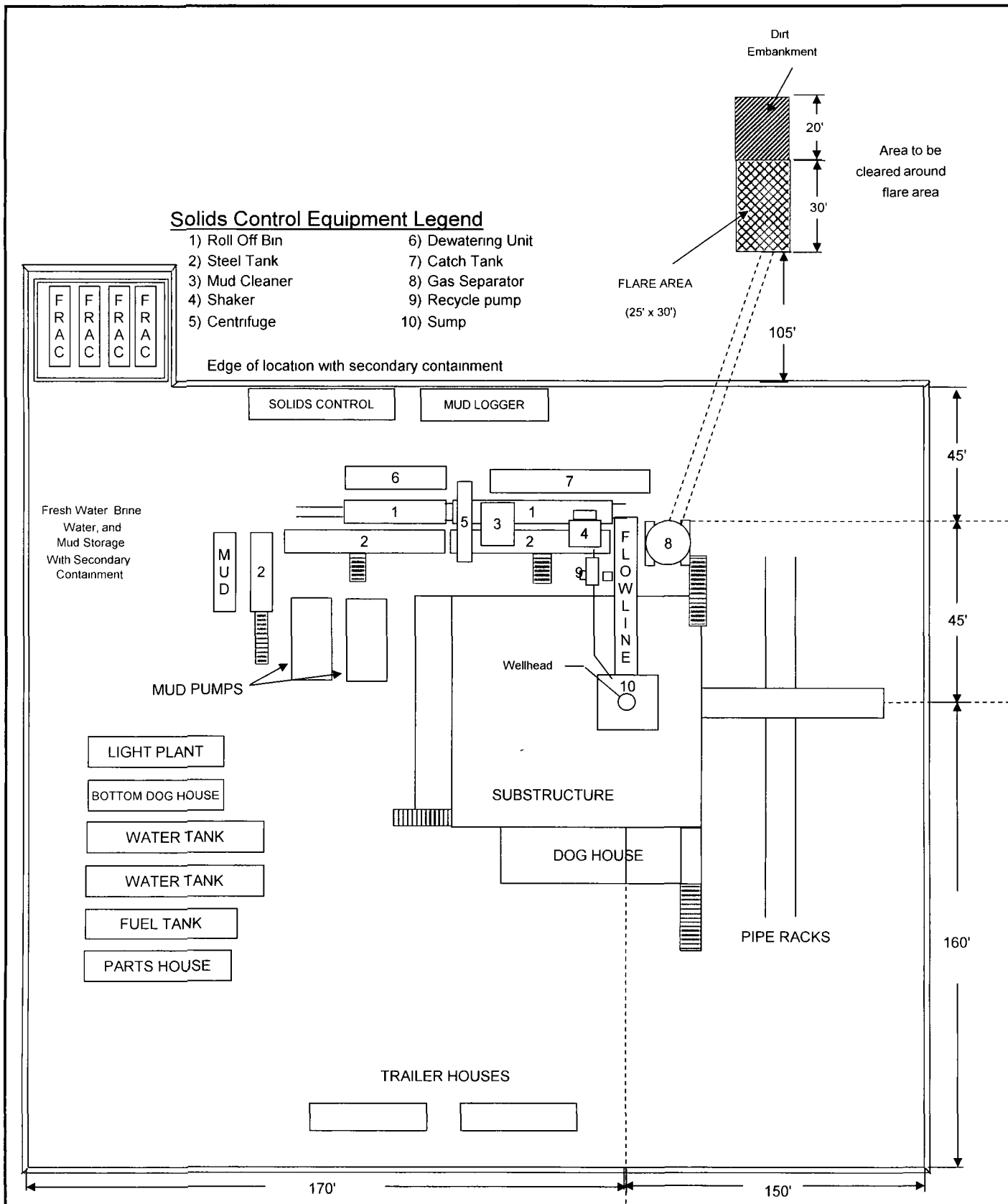
POKER LAKE UNIT 349H TYPICAL RIG LAYOUT SCHEMATIC INCLUSIVE OF CLOSED-LOOP DESIGN PLAN
