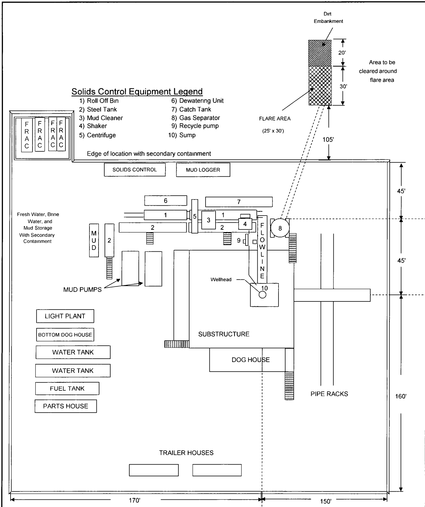
POKER LAKE UNIT 322H TYPICAL RIG LAYOUT SCHEMATIC INCLUSIVE OF CLOSED-LOOP DESIGN PLAN
