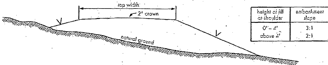
Embankment Section
