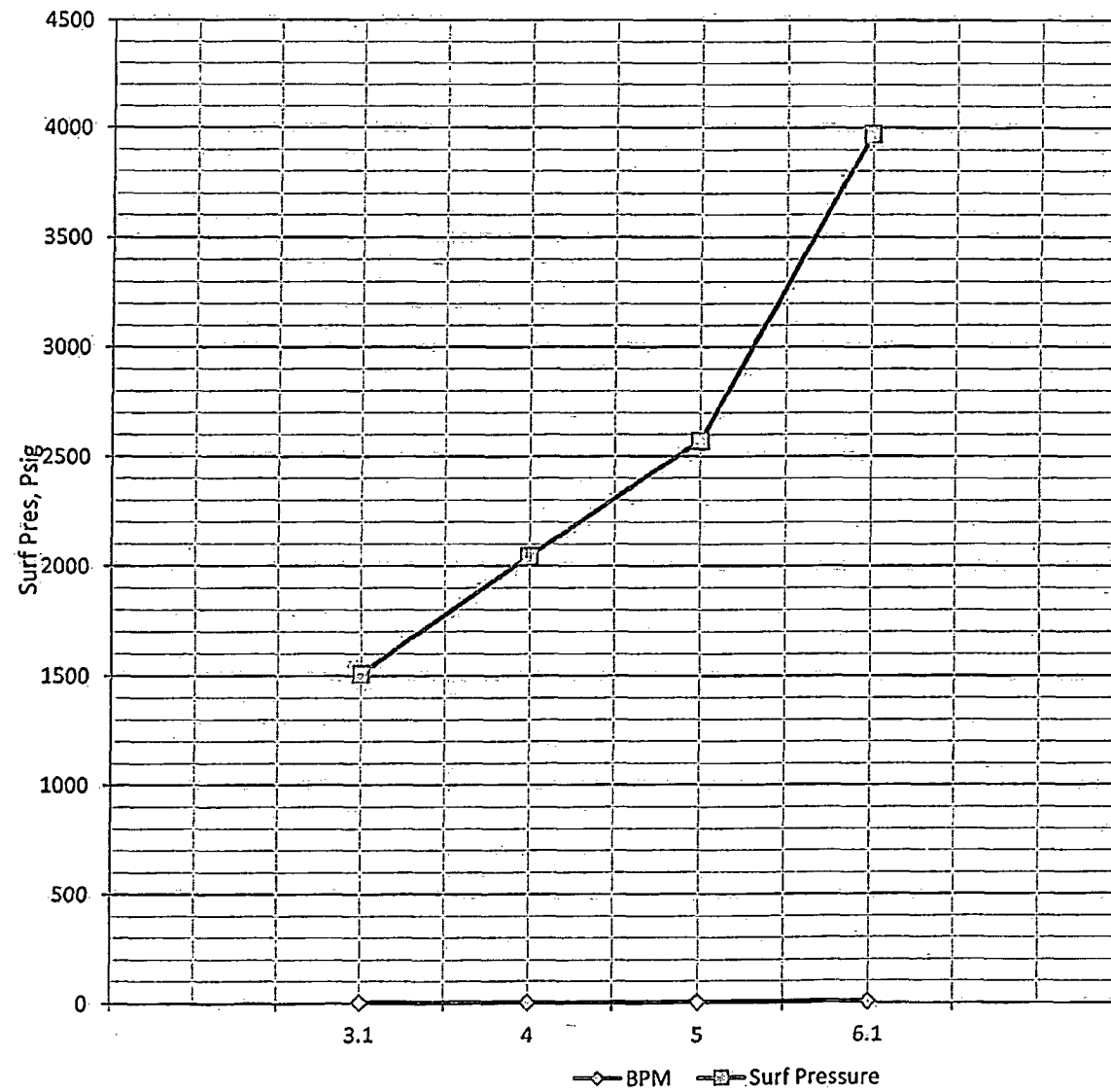
Apache St. SWD #1 - Step-Rate Injectivity - Surf Pres (4 1/2" x 3 1/2" x 2 1/2" Tapered Tubing String)
