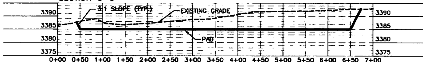
SECTION C-C'
