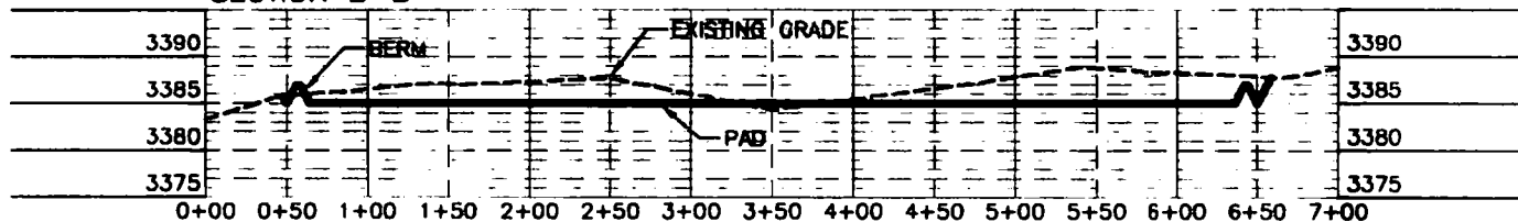
SECTION B-B'
