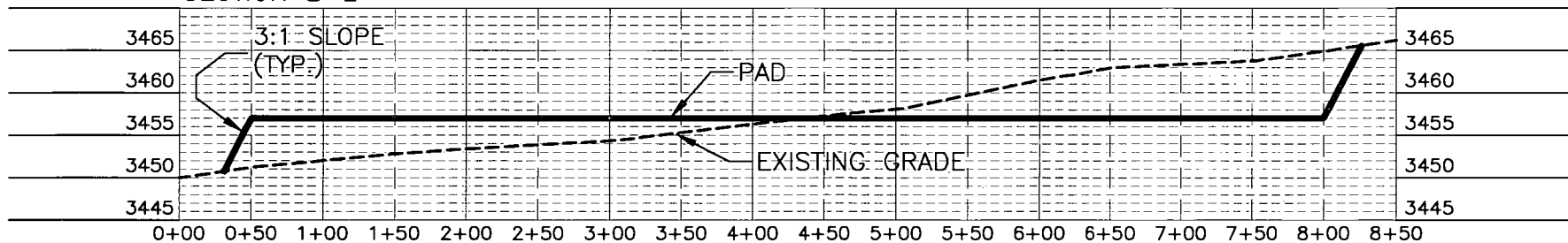
SECTION E-E'
