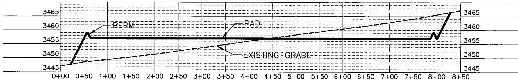
SECTION C-C'
