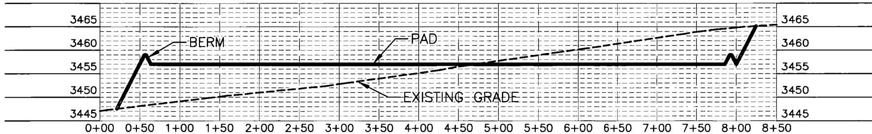
SECTION E-E'
