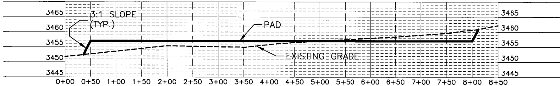
SECTION B-B'
