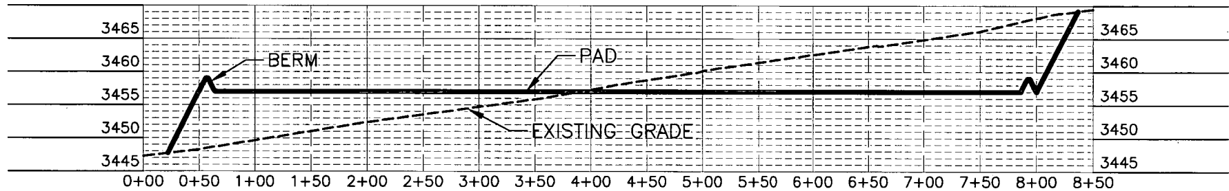
SECTION C-C'
