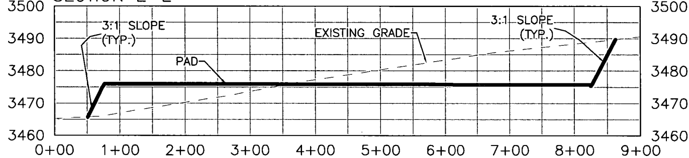
SECTION E-E
