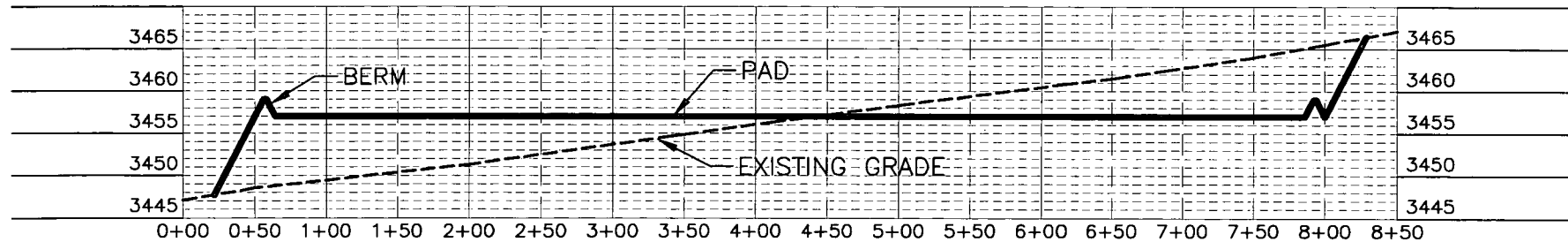
SECTION C-C'
