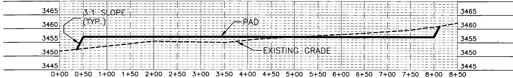
SECTION B-B'
