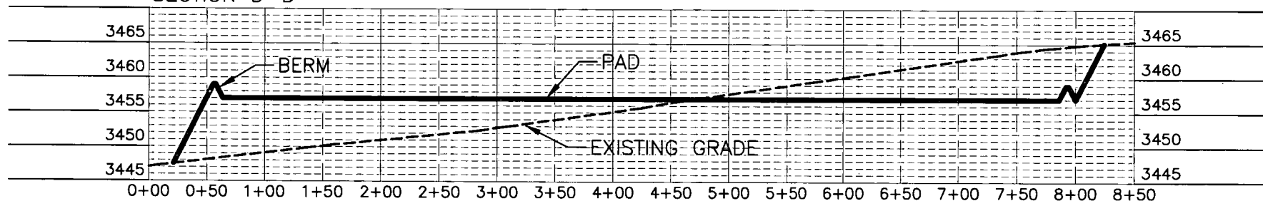
SECTION E-E'
