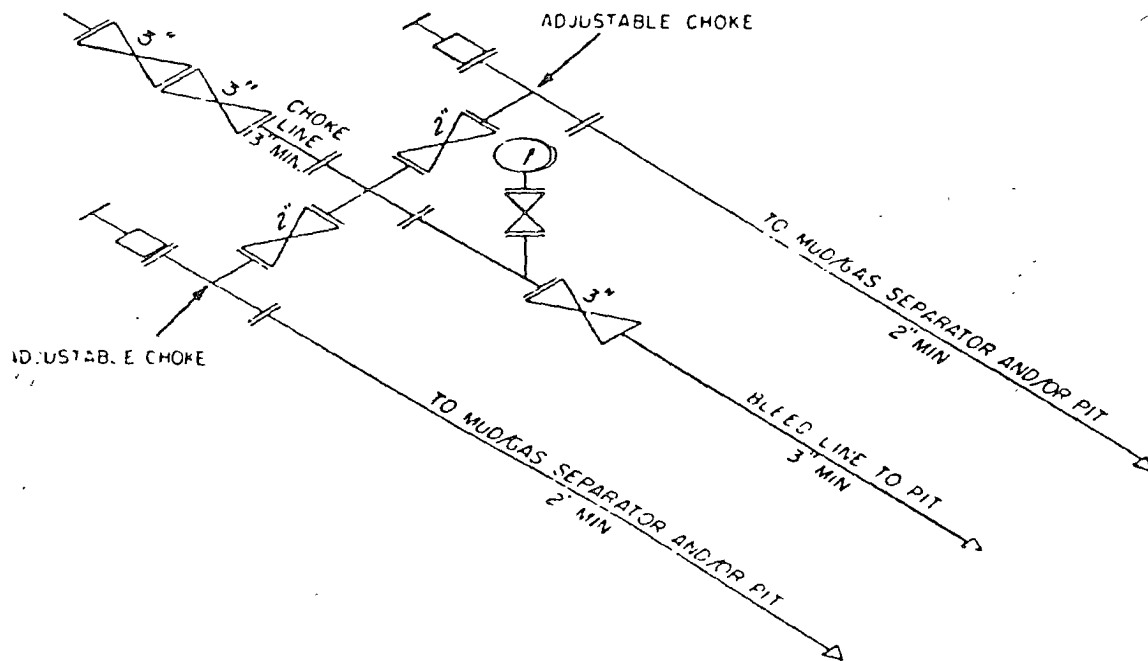
3M CHOKE MANIFOLD EQUIPMENT — CONFIGURATION OF CHOKES
