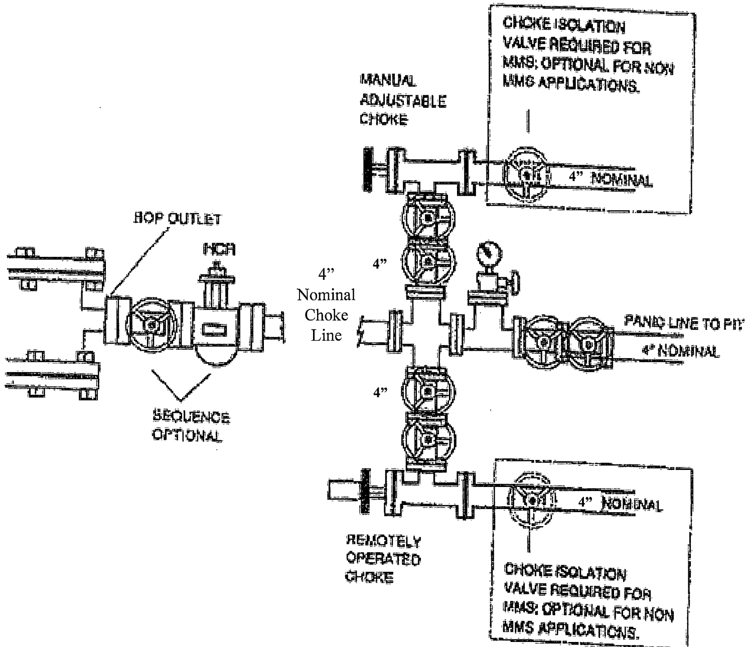
Exhibit E-1 – Choke Manifold Diagram Nitro 11 Federal Com No. 4 Cimarex Energy Co. of Colorado 11-16S-29E 390' BHL SHL 660' FSL & 330' FWL BHL 660' FSL & 330' FEL Eddy County, NM
