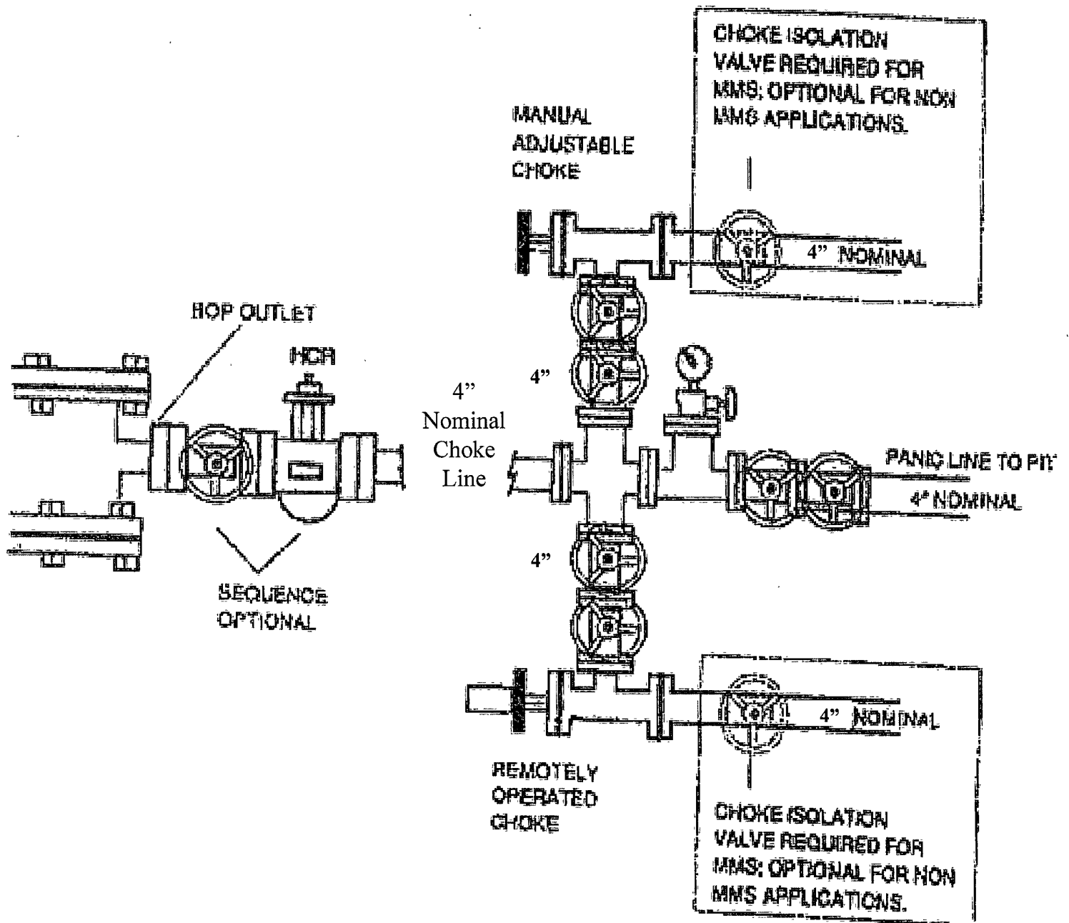
Exhibit E-1 – Choke Manifold Diagram Conoco 22 Federal Com No. 4 Cimarex Energy Co. of Colorado 22-16S-29E SHL 375 FNL & 330 FEL BHL 375 FNL & 330 FWL Eddy County, NM
