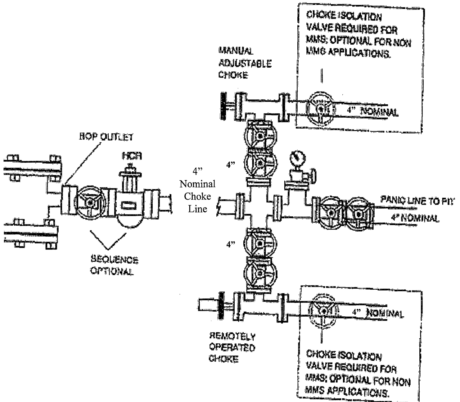
Exhibit E-1 – Choke Manifold Diagram County Line 1 Federal No. 2 Cimarex Energy Co. of Colorado 1-16S-29E SHL 330 FSL & 330 FWL BHL 330 FSL & 330 FEL Eddy County, NM
