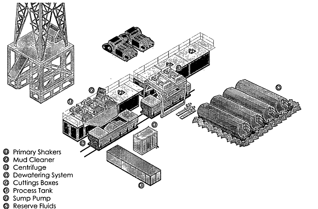
Closed Loop Schematic
