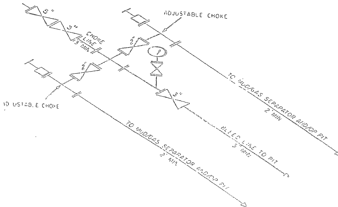
3M CHOKE MANIFOLD EQUIPMENT — CONFIGURATION OF CHOKES
