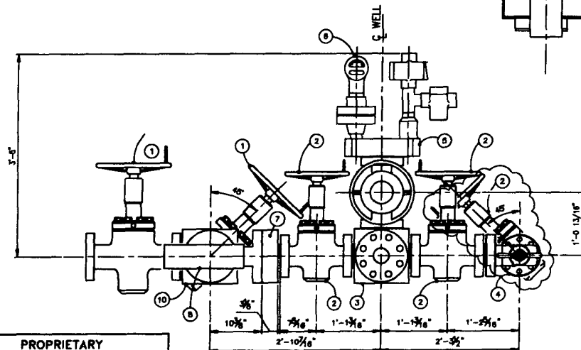
ELEVATION VIEW
