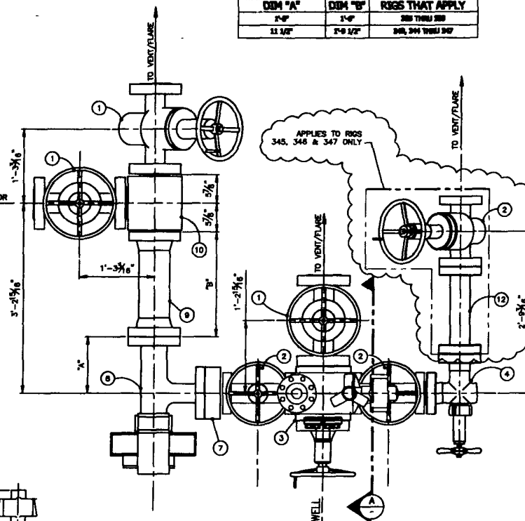
PLAN VIEW CHOKES MANIFOLD
