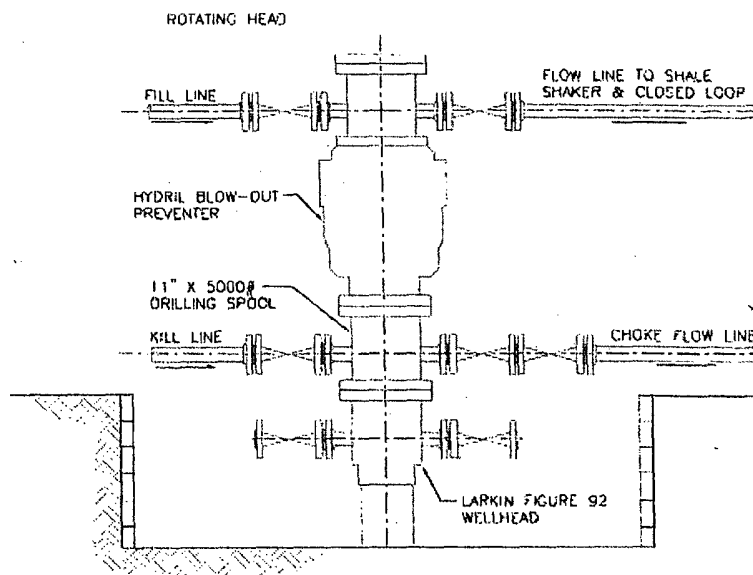
WELLHEAD ELEVATION
