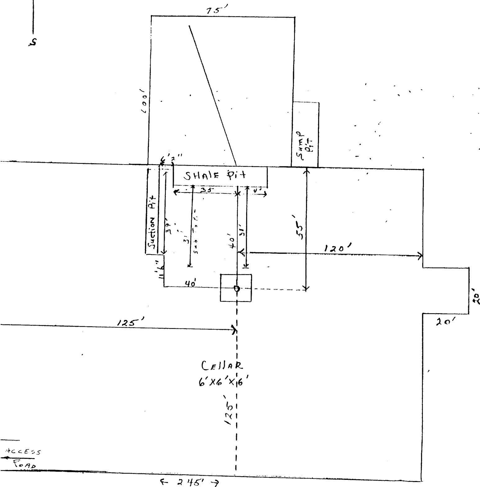
EXHIBIT "D" CHI OPERATING, INC. Remington Federal, Well No. 2 Pad & Pit Layout
