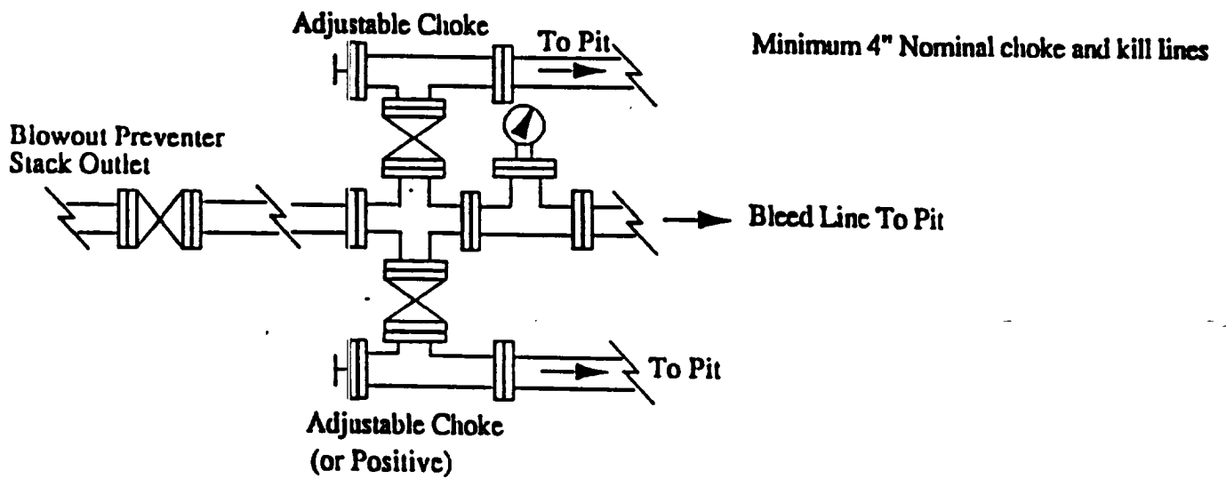
Choke Manifold Requirement ( 3000 psi WP)
