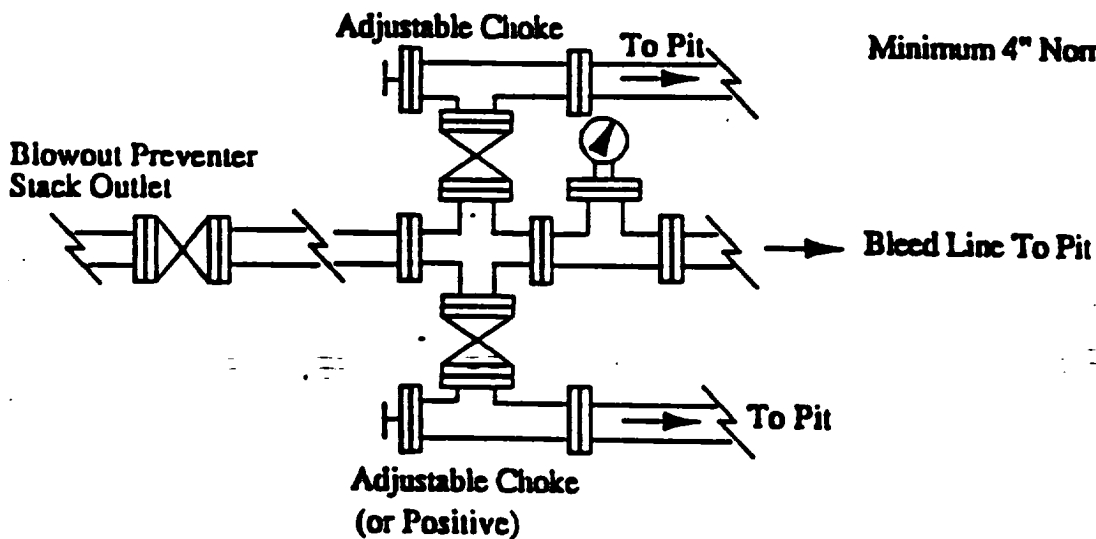
Choke Manifold Requirement ( 3000 psi WP)
