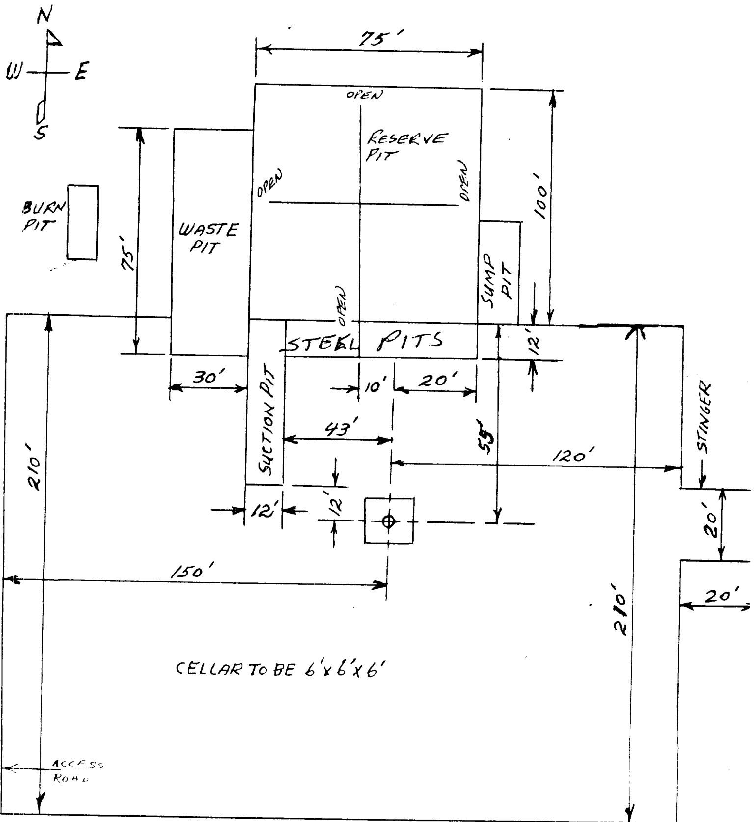
EXHIBIT "D" BILL FENN, INC. Lucky Stiff Federal, Well No. 1 Rig Layout
