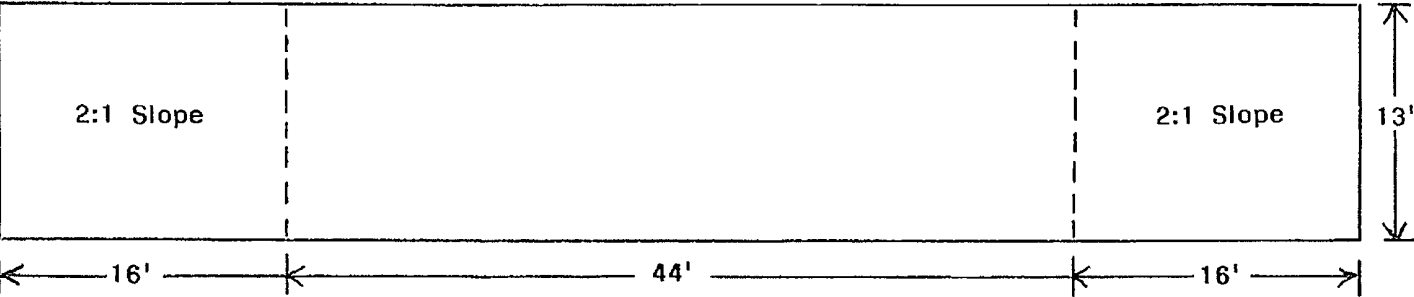
PLAN VIEW
