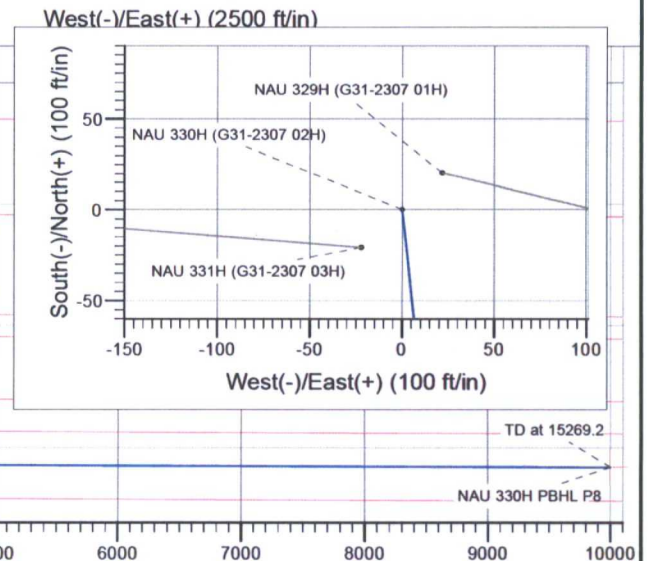
Vertical Section at 311.72° (1500 ft/in)
