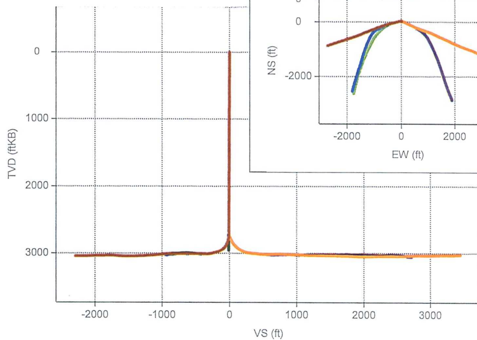
Vertical Section
