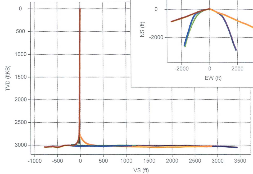
Vertical Section
