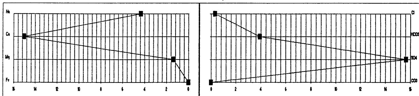
Stiff Diagram
