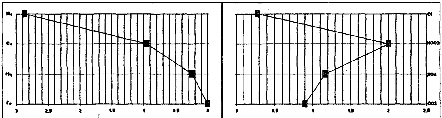
Stiff Diagram
